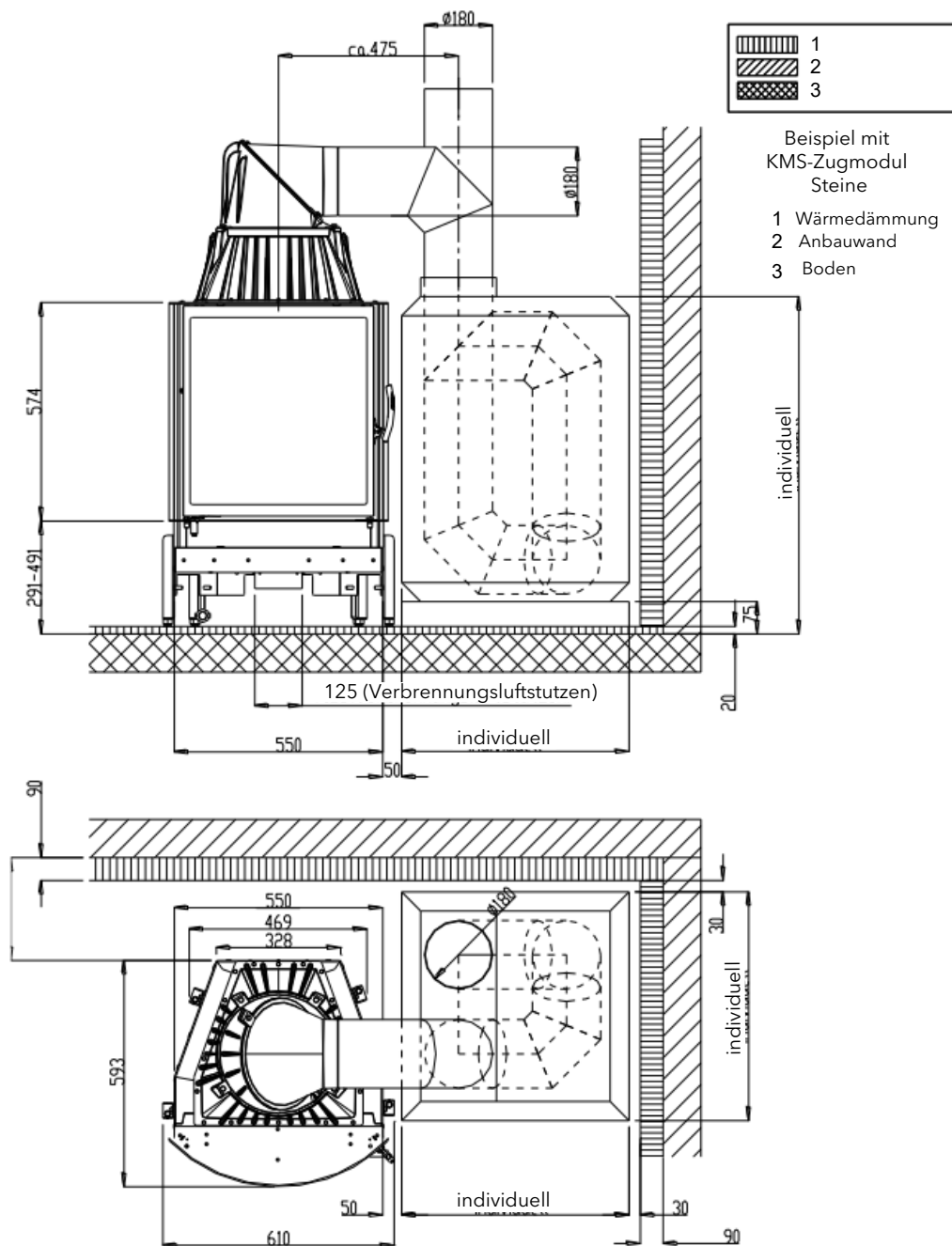
Abb. 15: KMS System
