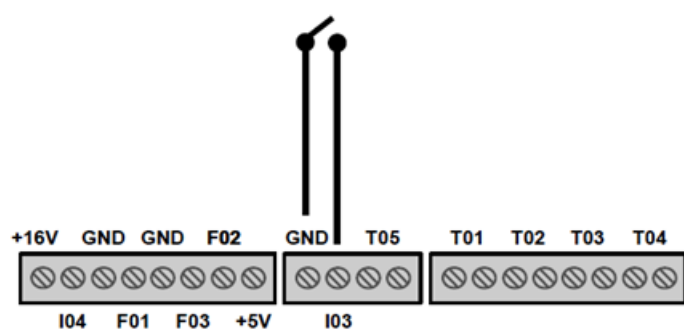
Abb. 19: Externer Thermostat
